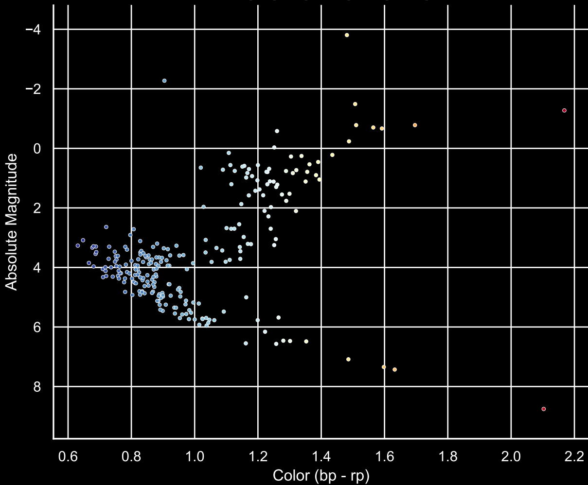
GALAH Hertzprung-Russel Diagram Field [113] Ra [320.05] Dec [-22.22]
