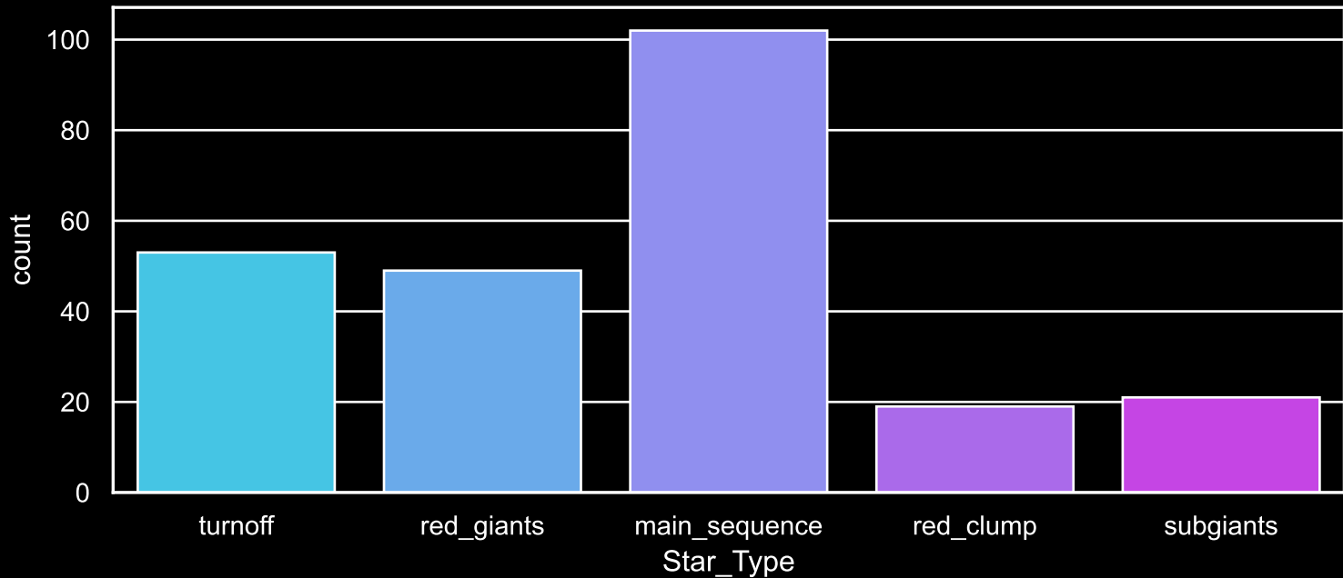
Field [113] Count plot of Star Type
