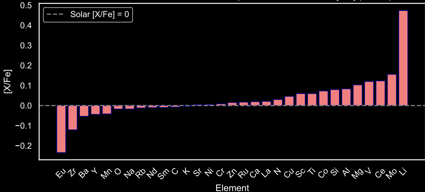
Abundance Pattern for GALAH Main Sequence Stars: Star Field [113] (N=102)
