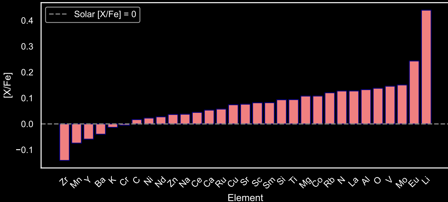
Abundance Pattern for GALAH Star Field [113] (N=244)
