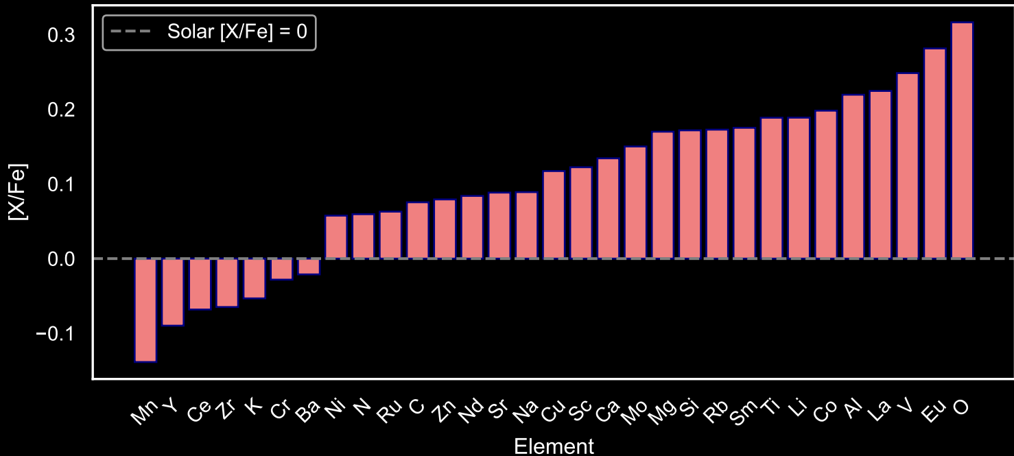
Abundance Pattern for GALAH Red Giants: Star Field [113] (N=68)
